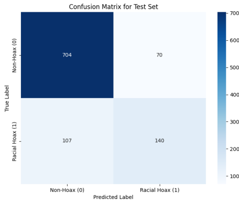
Figure 3: Confusion matrix of the proposed model (fine-tuned HingRoBERTa-Mixed) on test set
